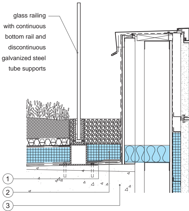
As-Built Condition
