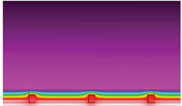
Studs pulled 1" back from existing wall 16% of baseline calculated R-value
