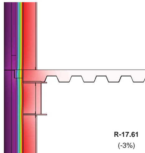
Discontinuous Stainless Shelf Angle
