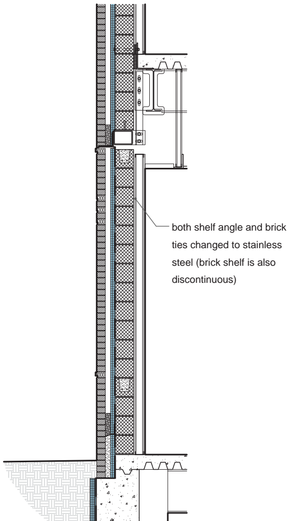
Digital Image
