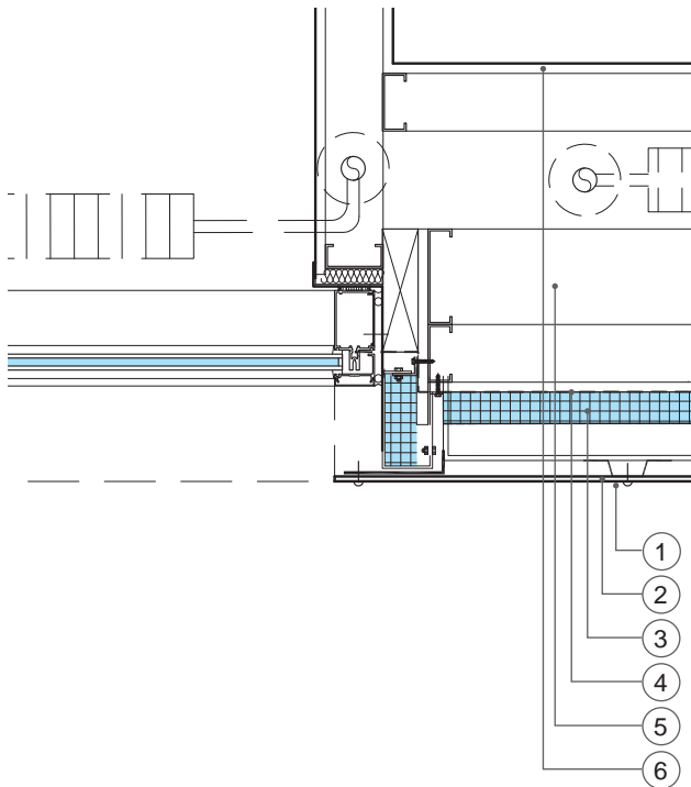
As-Built Condition
