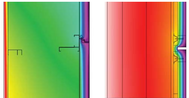
Metal Panel w/ Uninsulated Joints
