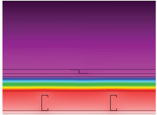
Studs separated from insulation 2% of baseline calculated R-value
