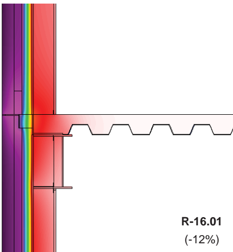
Discontinuous Galvanized Shelf Angle
