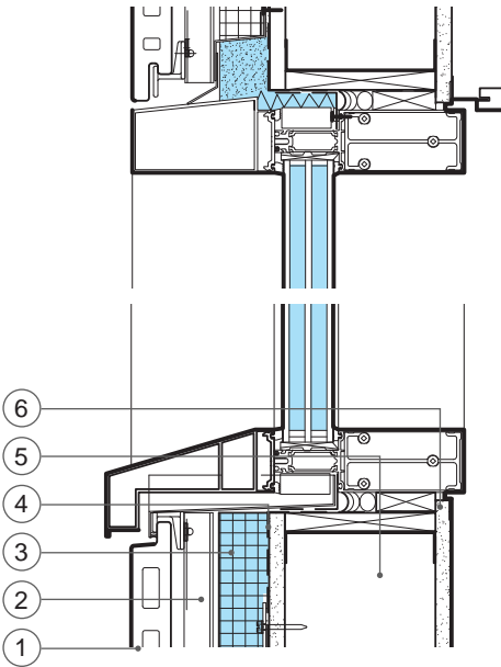
Section Detail
