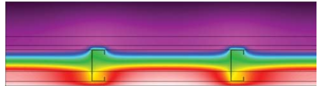
Studs directly attached to existing wall 59% of baseline calculated R-value
