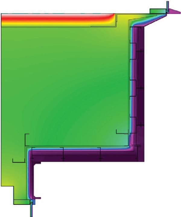
Thermally Improved Condition
