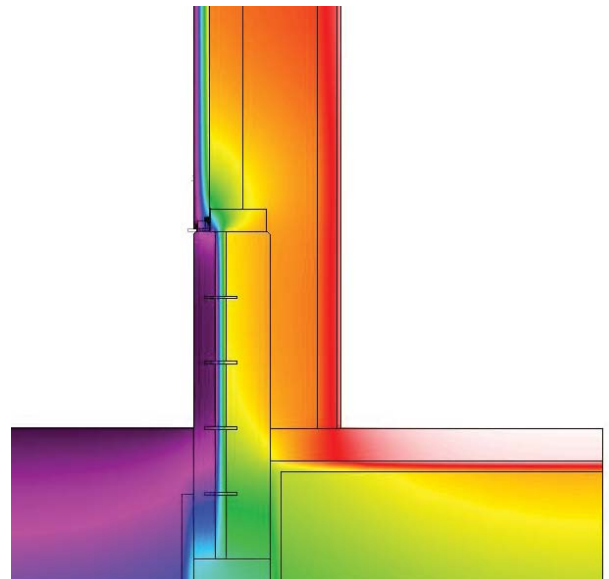
R-9.82 (wall), R-18.36 (floor) (+139% wall, +68.8% floor)
