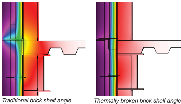
Traditional brick shelf angle
