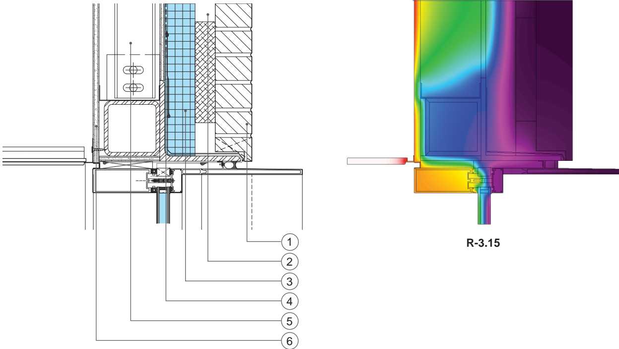
As-Built Condition
