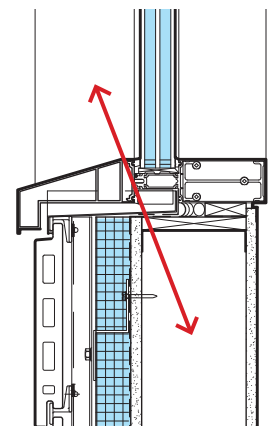
Window in-line with insulation
