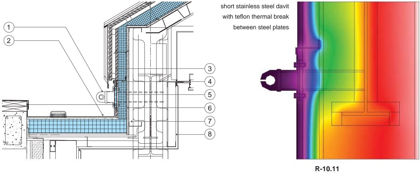
As-Built Condition
