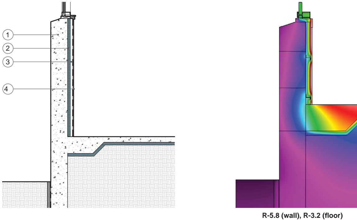
As-Built Condition
