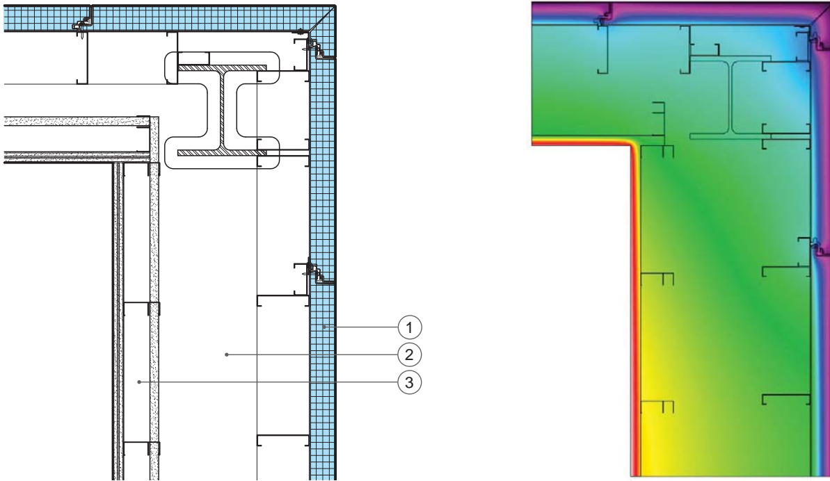
As-Built Condition
