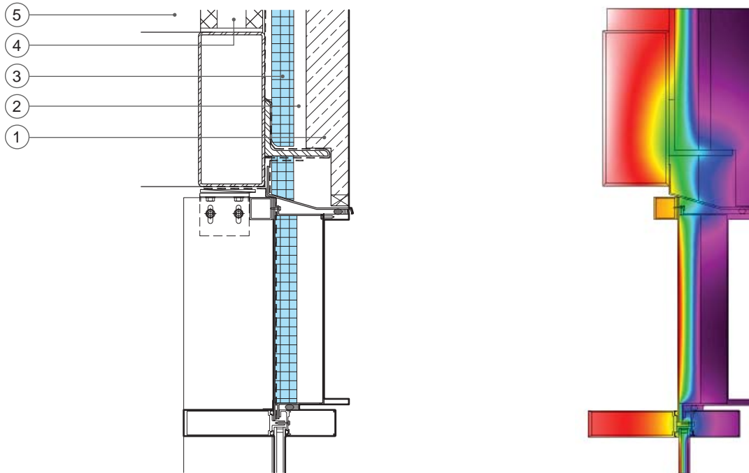
As-Built Condition
