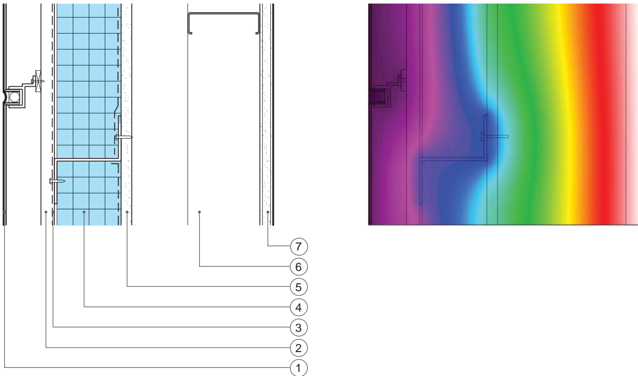
As-Built Condition
