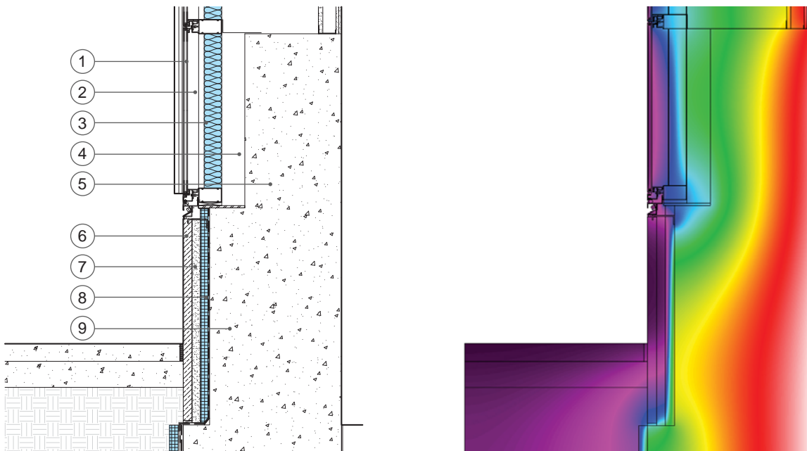
As-Built Condition
