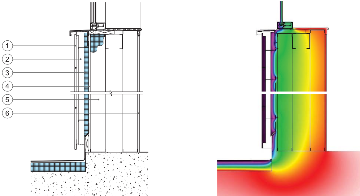
As-Built Condition
