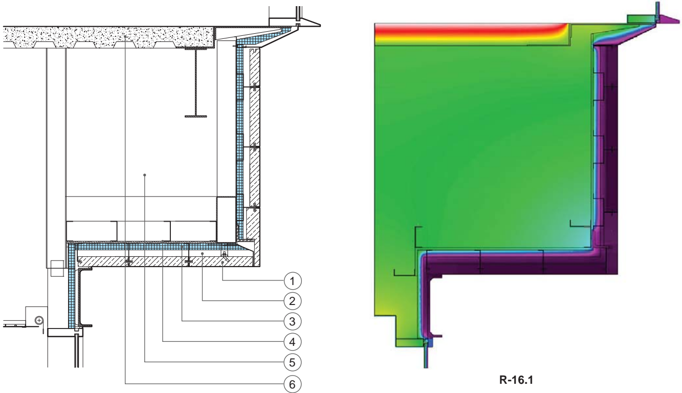
As-Built Condition
