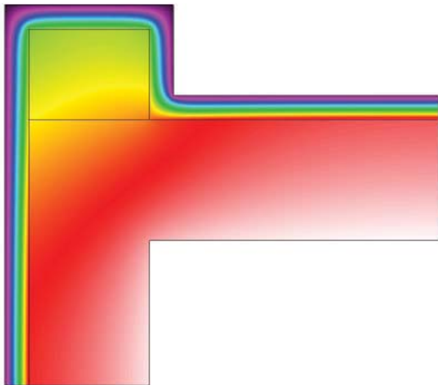
R-13.42 Insulating around 1'-3" tall parapet
