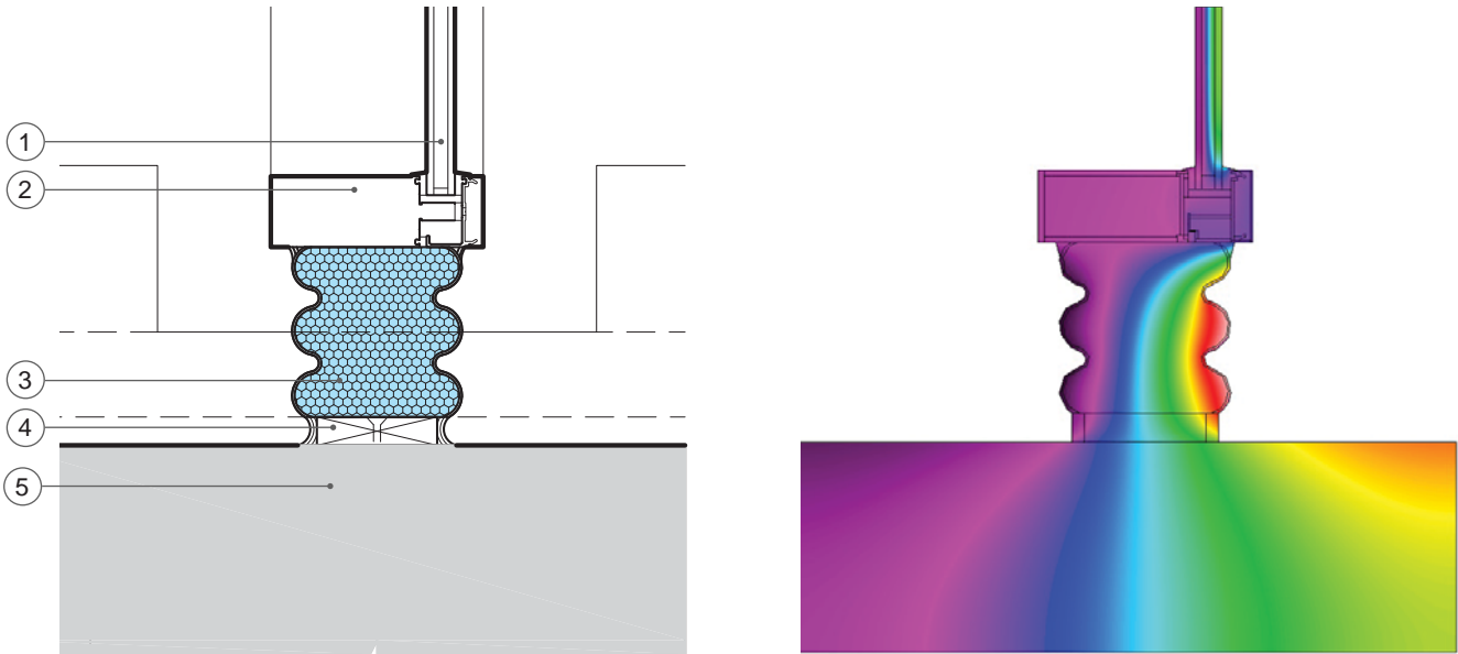
As-Built Condition
