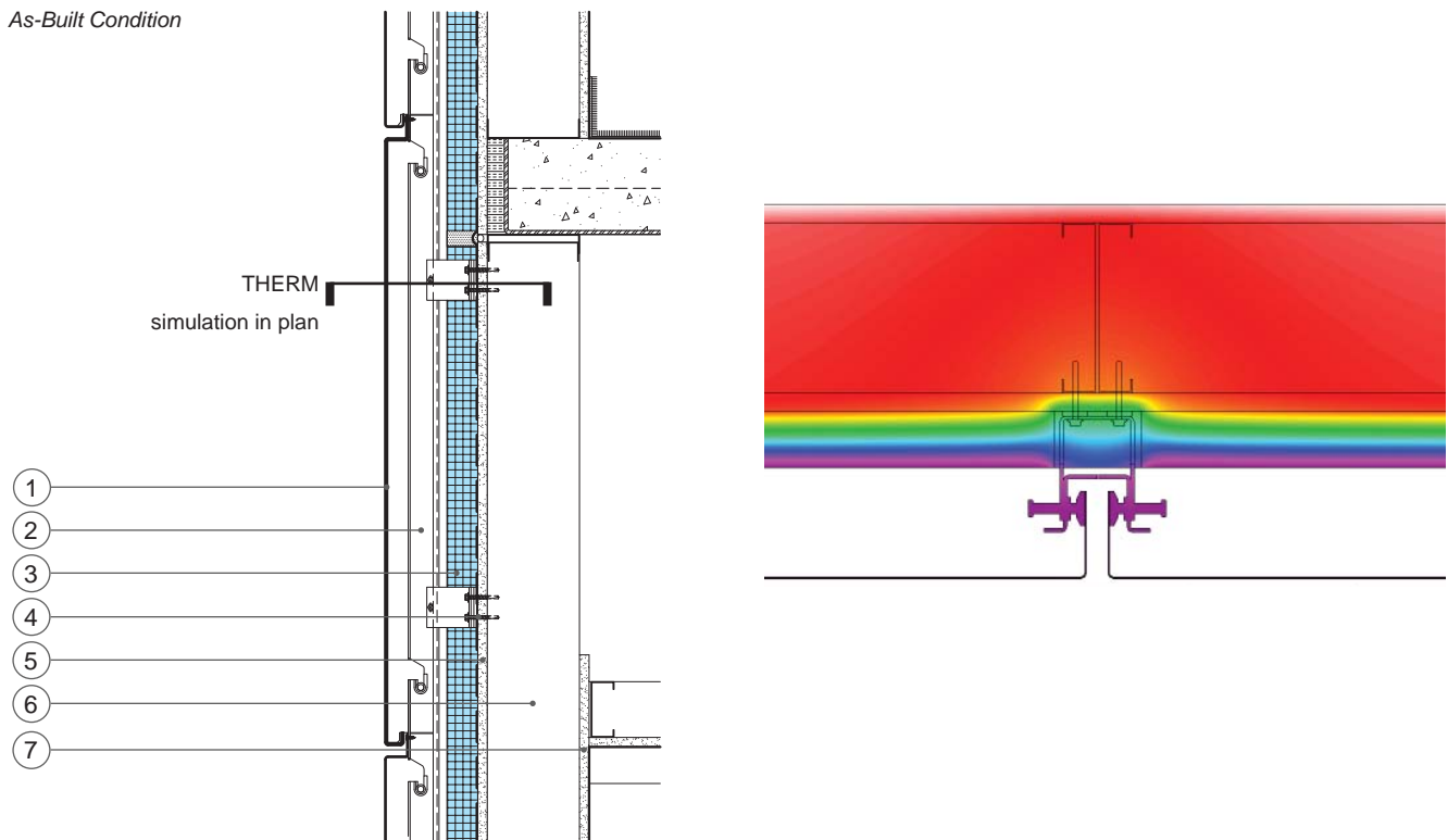
As-Built Condition
