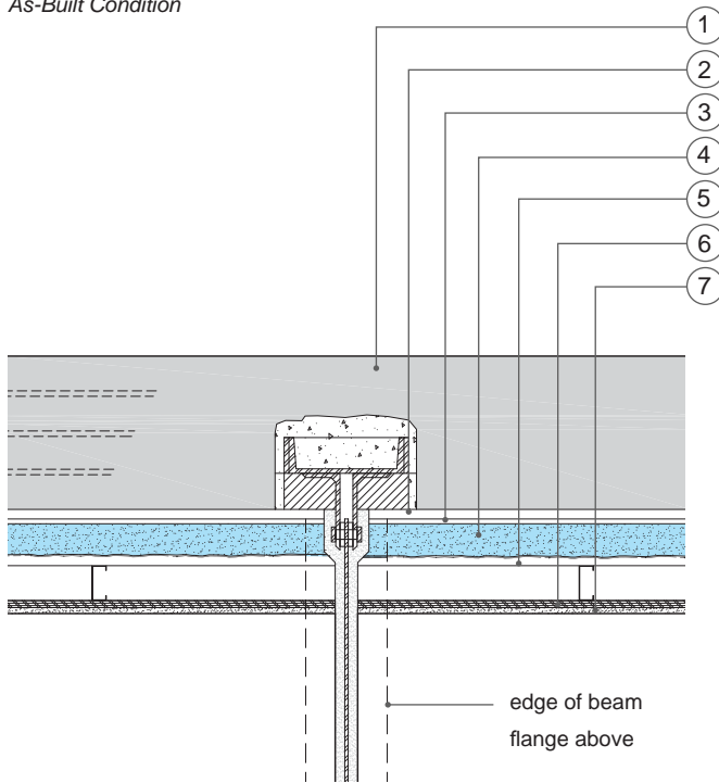
As-Built Condition
