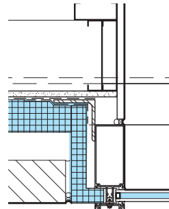
Plan Detail
