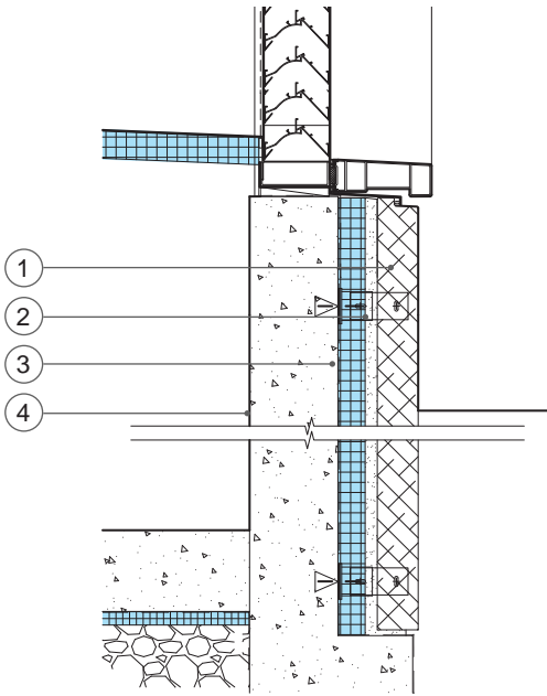
As-Built Condition
