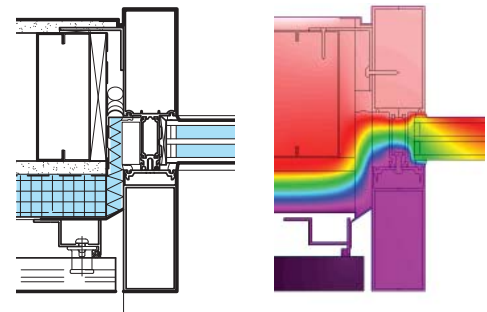
Plan Detail
