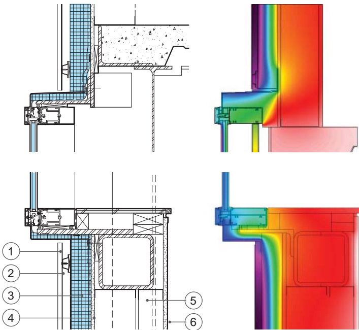
Section Detail
