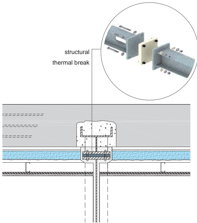
Digital Image
