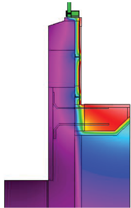
R-6.1 (wall), R-5.85 (floor) (+5% wall, +82.8% floor)
