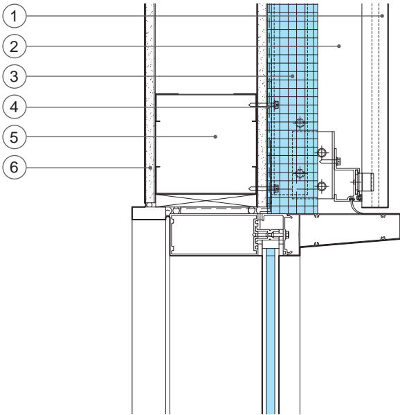
As-Built Condition
