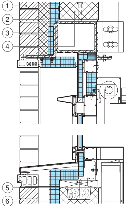
Section Detail
