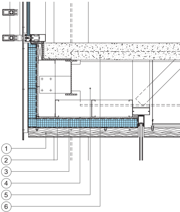
As-Built Condition
