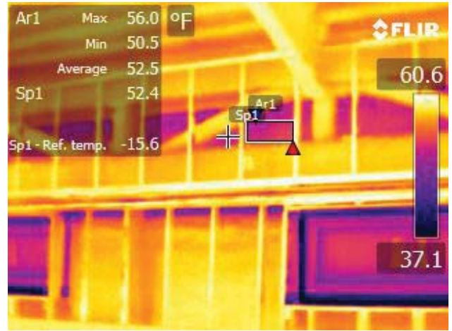
Infrared Image
