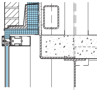
Section Detail
