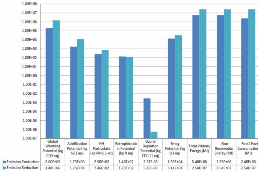
Figure 9: Comparison between produced and reduced emission through the process of Grayson Hall renovation.
