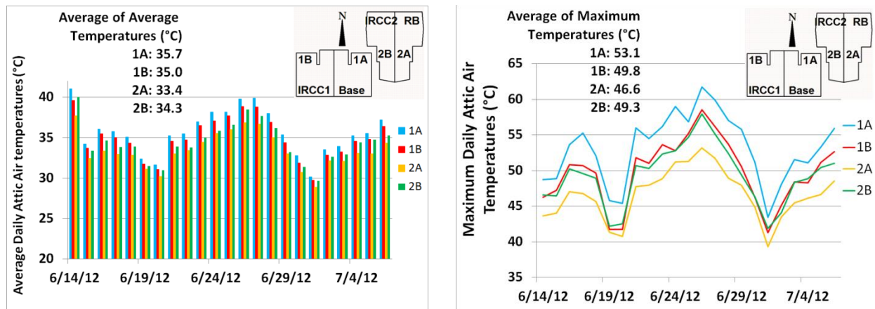
Figure 5: Average daily attic air temperatures recorded in four test attics (center location) during the June/July measure period (Left); Maximum daily attic air temperatures recorded in four test attics (center location) during the June/July measure period (Right)
