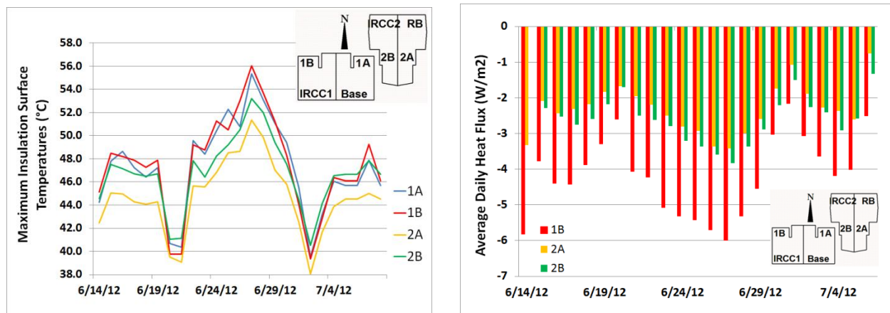
Figure 7: Maximum daily temperatures on the top surface of the attic insulation recorded in three test attics using radiation control technologies and a conventional base case, during the June/July measure period (Left); Heat fluxes recorded in test attics using radiation control technologies and a conventional base case, during the June/July measure period. Positive heat flow direction is from conditioned space to the attic (Right).
