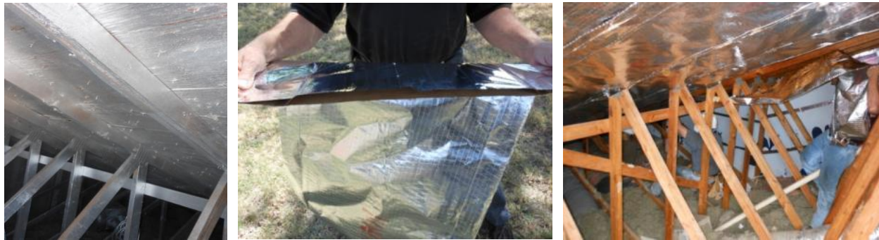
Figure 3: Installation of IRCC (left) & RB with enclosed airspace underside of the roof deck (middle, right)
