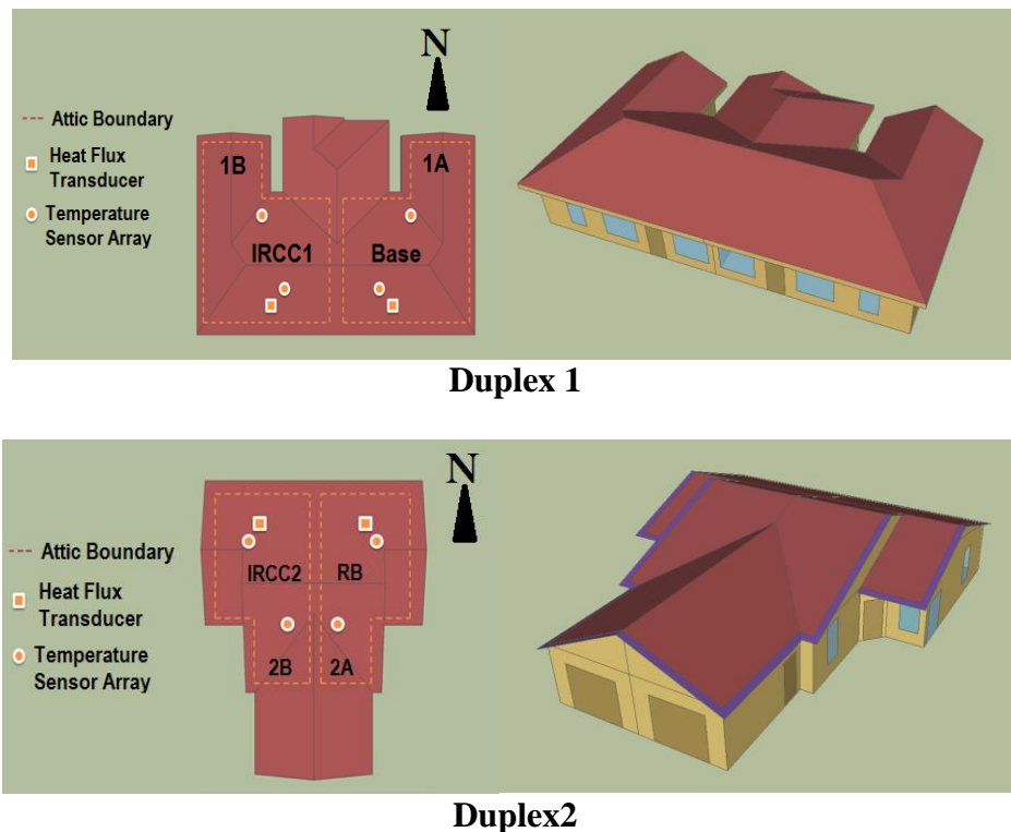
Figure 1: Location of thermistor arrays and heat flow transducers inside the tested attics
