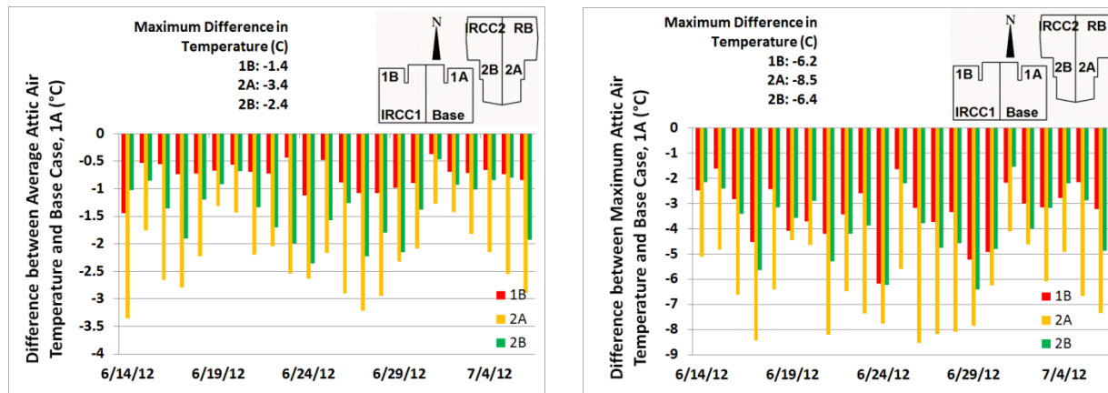
Figure 5: Differences in average daily attic air temperatures recorded between three test attics using radiation control technologies and a baseline attic, during the June/July measure period (Left); Differences in maximum daily attic air temperatures recorded between three test attics using radiation control technologies and a baseline attic, during the June/July measure period (Right)
