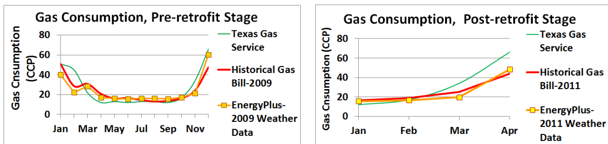
Figure 8: Comparison of monthly historical gas bill, simulated consumption, and the gas consumption by Texas Gas Service calculator. Gas consumptions are for duplex 1B before (Left) and after (Right) installing radiation control technology. The EnergyPlus simulation is based on actual weather file data from 2009 (before retrofit) and 2011 (after retrofit).
