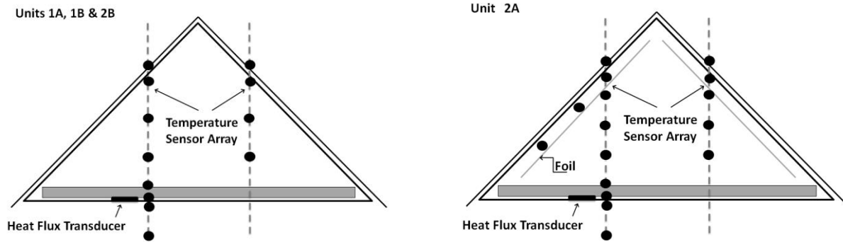
Figure 2: Diagrams of the attic sensor distributions for a RB combined with an enclosed reflective air space (right diagram), and IRCC and baseline (left diagram).
