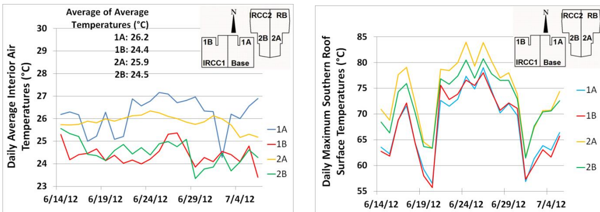
Figure 4: Average interior air temperatures recorded during the June/July measure period (Left); Maximum roof surface temperatures recorded during the June/July measure period (Right).
