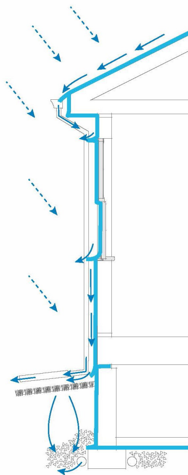
Graphic 1. Example continuous water control layer (indicated by solid blue line) and water draining down and away from the building (solid blue arrows) [2].
