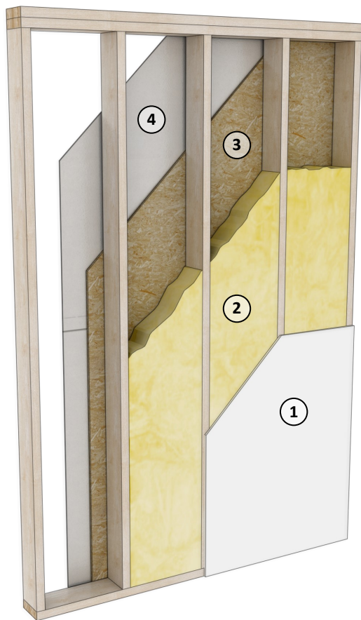
Figure 3. Wall Assembly without Vapor Retarder
