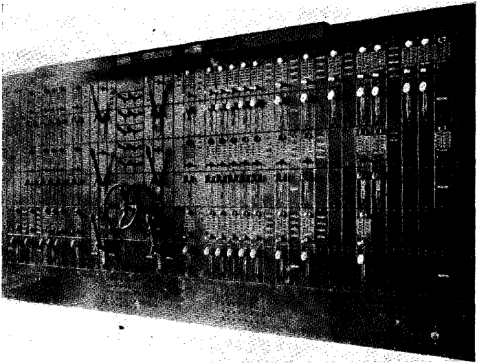
FIG. 1—A typical ten-scene switching preset Major control board built by the Frank Adam Electric Company of St. Louis.
